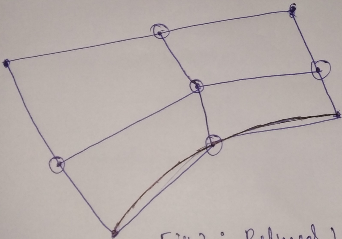
Fig 1 : Quadratic Mesh
