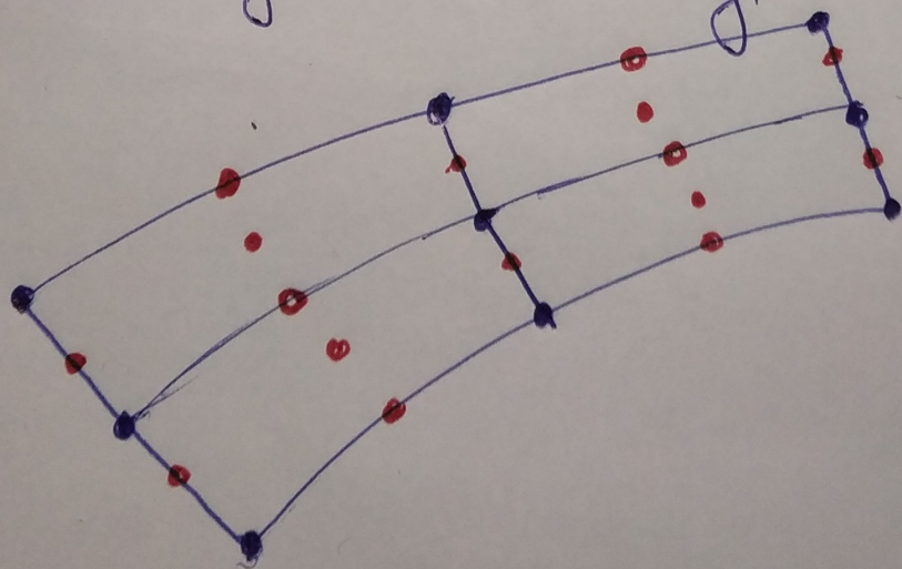
Fig-3 Desired Mesh after one refinement. (quadratic-degree 2)
